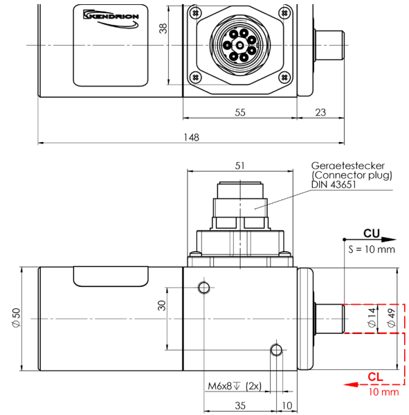
Dimension drawing
