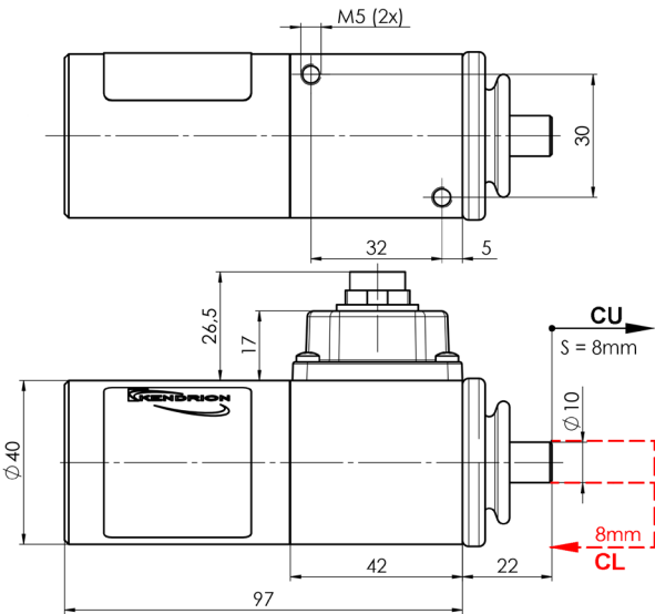
Dimension drawing
