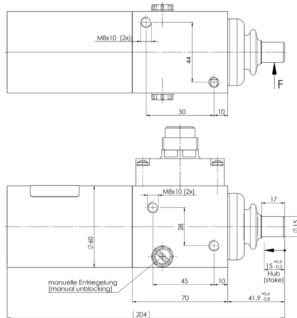
Dimension drawing
