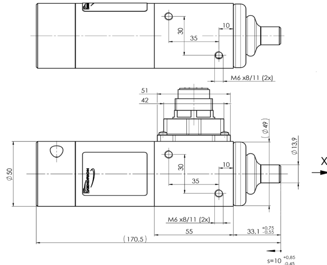
Dimension drawing
